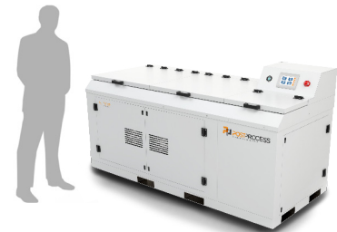
NITOR Envelope: 60" x 24" x 20" 152.4 cm x 60.9 cm x 50.8 cm
